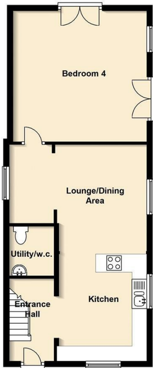
Ground Floor Approx. 67.1 sq. metres (722.3 sq. feet)
